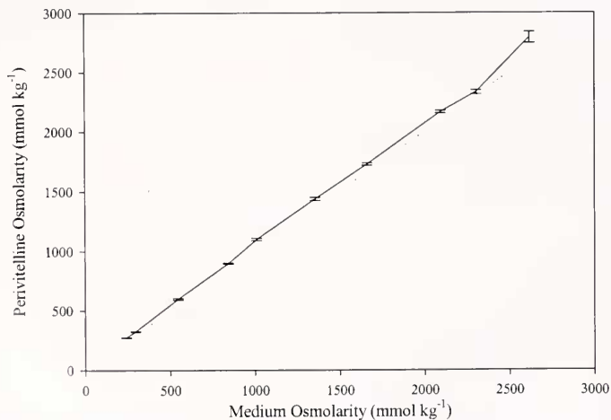
Figure 6. Variations in the perivittelline osmolarity of Limulus polyphemus eggs as a function of the bathing medium following 6 h of exposure. Values are means ( \pm SE). The dashed line is the isoosmotic line.
